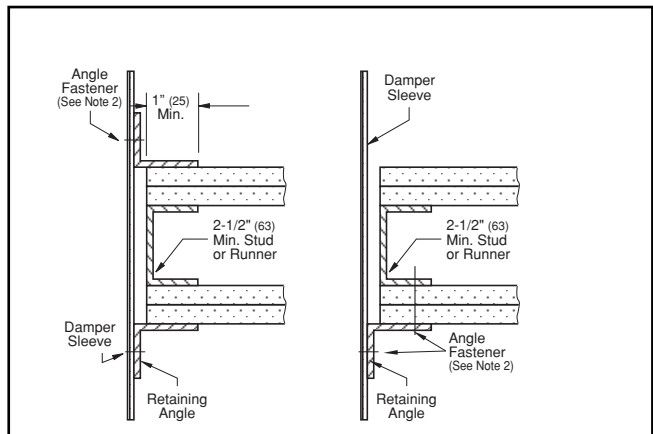
Wall with Two Layers of Drywall
