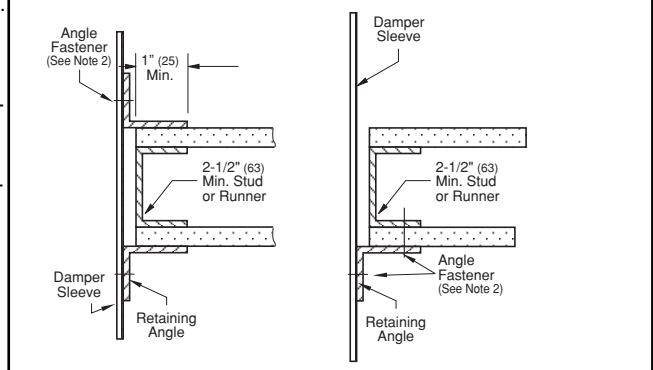
Wall with Single Layer of Drywall
