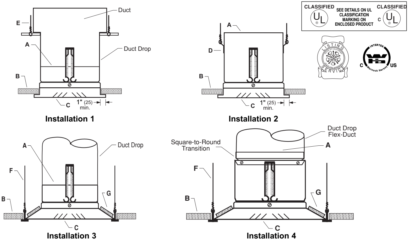
Illustrations show CFD-15 type damper, model CFD-20 similar.
